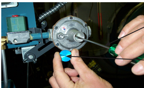
Figure E-6 Gas Pilot Regulator Adjustment
