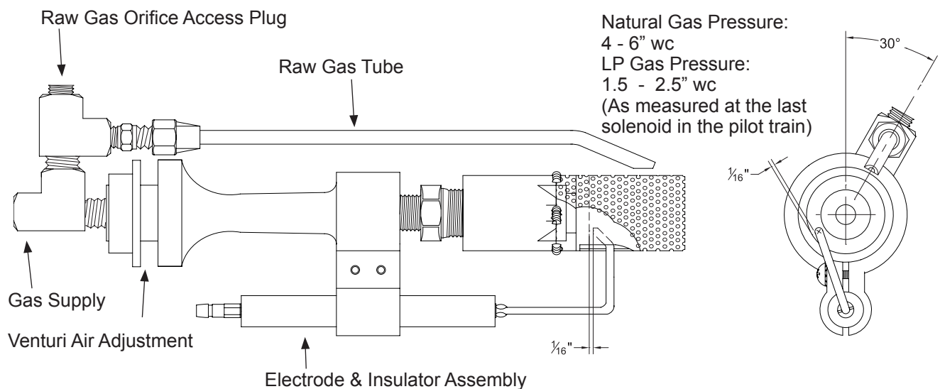
Figure E-5A JBS3 PILOT ASSEMBLY
