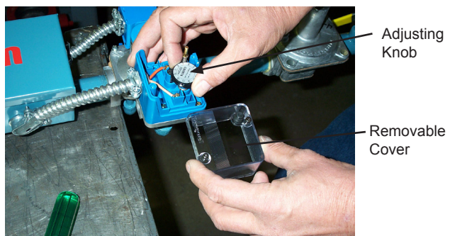
Figure E-8 Gas Pressure Switch Adjustment
