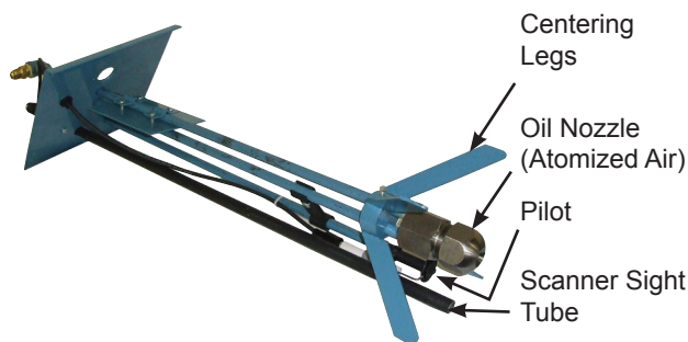
Figure B-8 Burner Drawer Assembly
