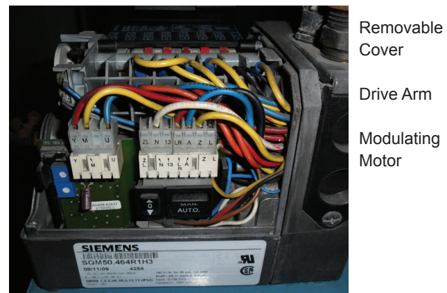
Figure B-18 Siemens Mod Motor Adjustments
