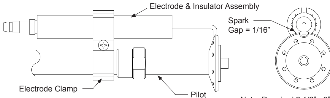
Figure E-5 JBS2 Gas Pilot
